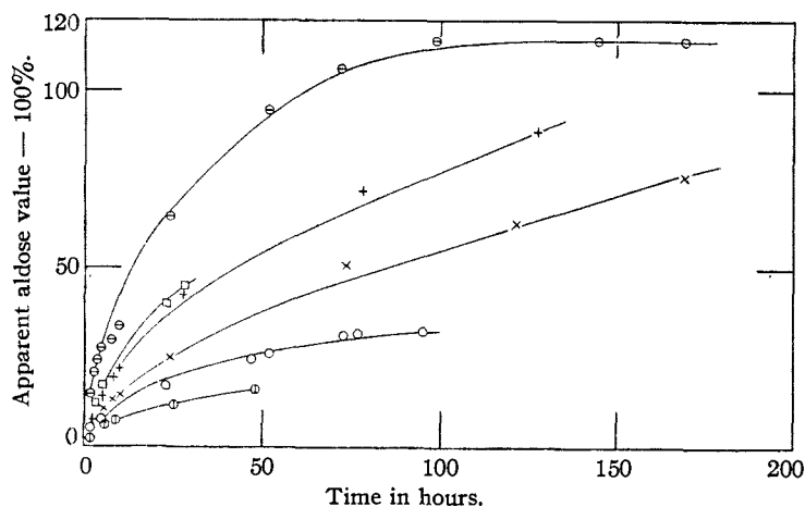
Fig. 2.—Rate of reaction of tetramethylglucose in dilute alkali: Expt. 1, \square ; Expt. 2, \circ ; Expt. 3, \times ; Expt. 4, + ; Expt. 5, \square ; Expt. 6, \ominus .
